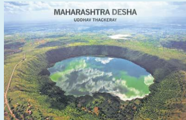
Crater formed in Maharashtra due to a meteorite crash
